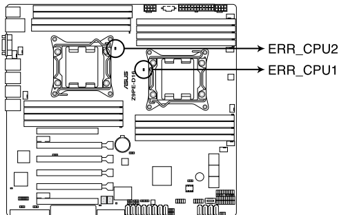
Z9PE-D16 Series ERR CPU LED
